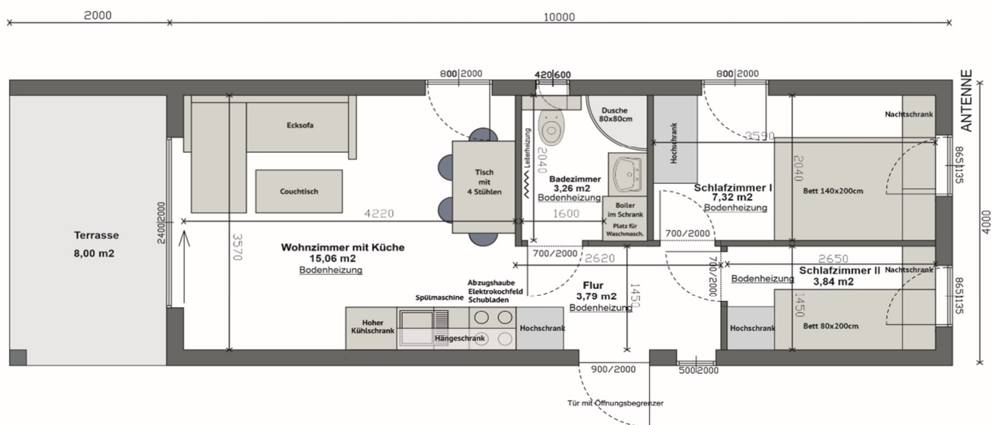
Grundriss MV48-4-B
